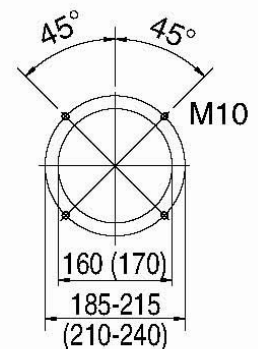
MGN 530 dimensions in brackets
